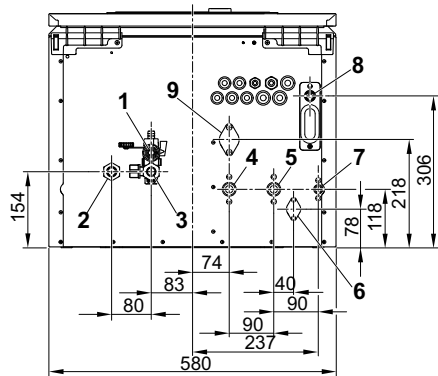
Abb. 11: WGB-K 22/28.1
