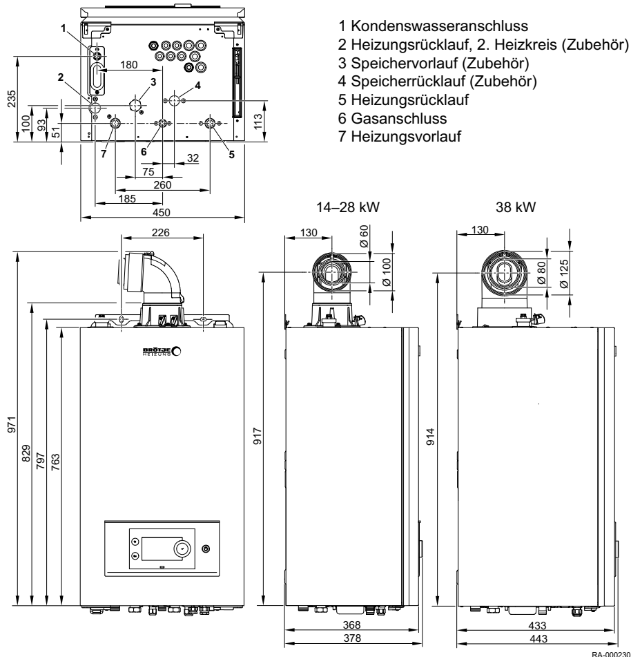
Abb. 8: WGB 14.1–38.1
